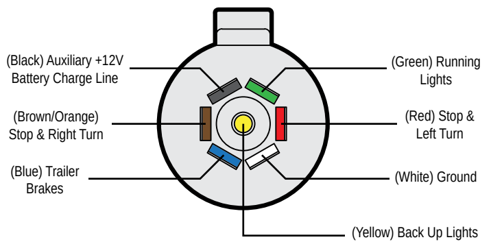
7-Way Trailer Plug (Cord End)
