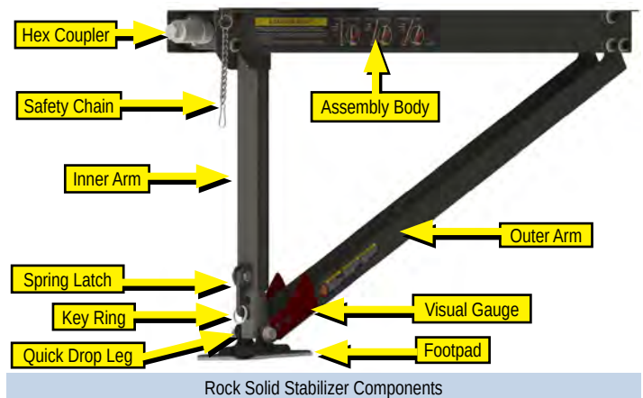
Rock Solid Stabilizer Components
