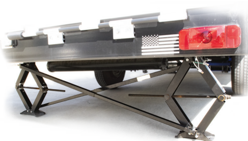
X-BRACE SCISSOR JACK STABILIZER
