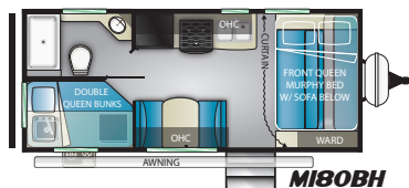
Length – 22' 9" Dry – 4,556 Hitch – 662
