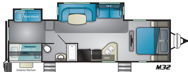
Length – 34' 10" Dry – 6,926 Hitch – 670
