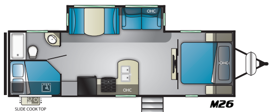
Length – 32' 1" Dry – 6,416 Hitch – 660
