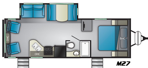
Length – 30' 4" Dry – 5,672 Hitch – 638
