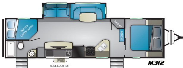
Length – 36' Dry – 7,012 Hitch – 672
